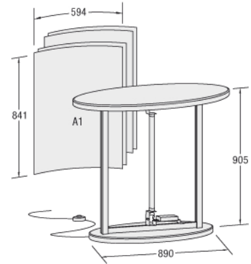
VA 7300 Basic set counter incl. illumination, 18 W / 230 V, and 4 panels A1 base and top cover: wood, silver
